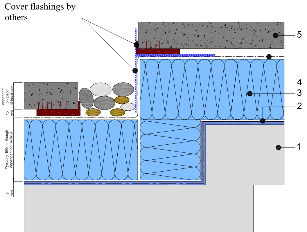
LEVEL CHANGE WITH STEP
